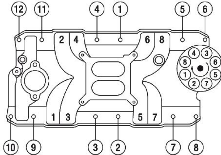
FIRING ORDER : 1-8-4-3-6-5-7-2
