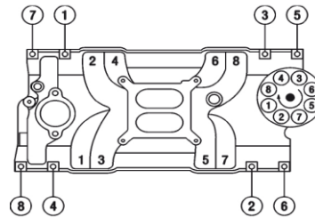
FIRING ORDER 1-8-4-3-6-5-7-2
