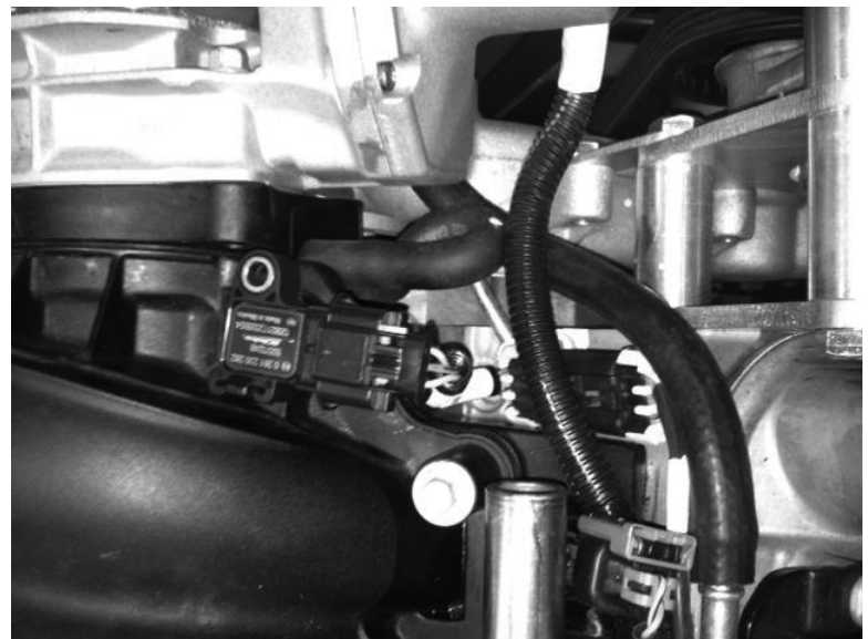
Figure 2 Re-install O’ring and install MAP sensor. Lubricate lightly with engine oil. Plug in MAP sensor using jumper provided with Engine control System kit. See Figure 3.
