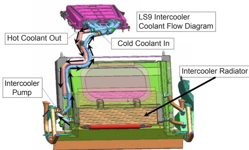
Typical Charge Air Cooler Set-Up
